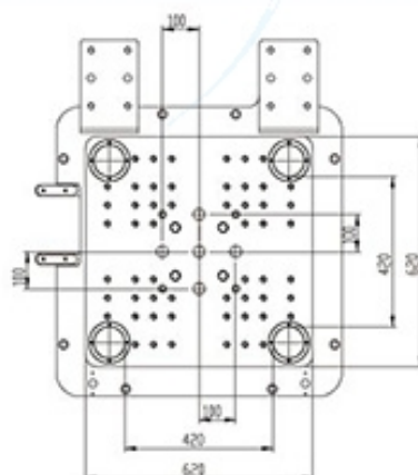
Stationary Platen
