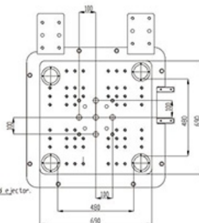
Stationary Platen
