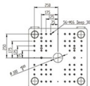
Moveable Platen
