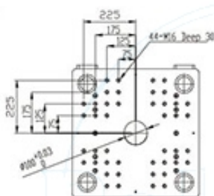
Moveable Platen
