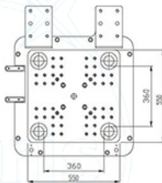
Stationary Platen
