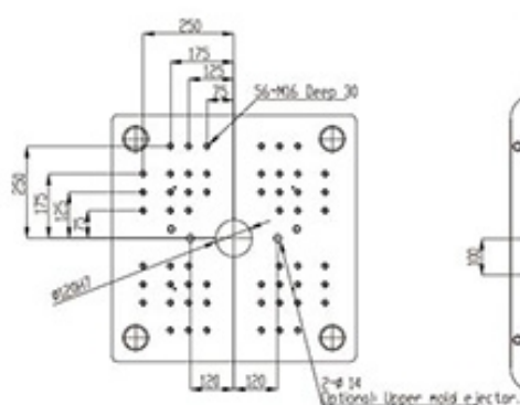
Moveable Platen
